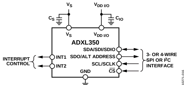
Figure 58. Application Diagram
